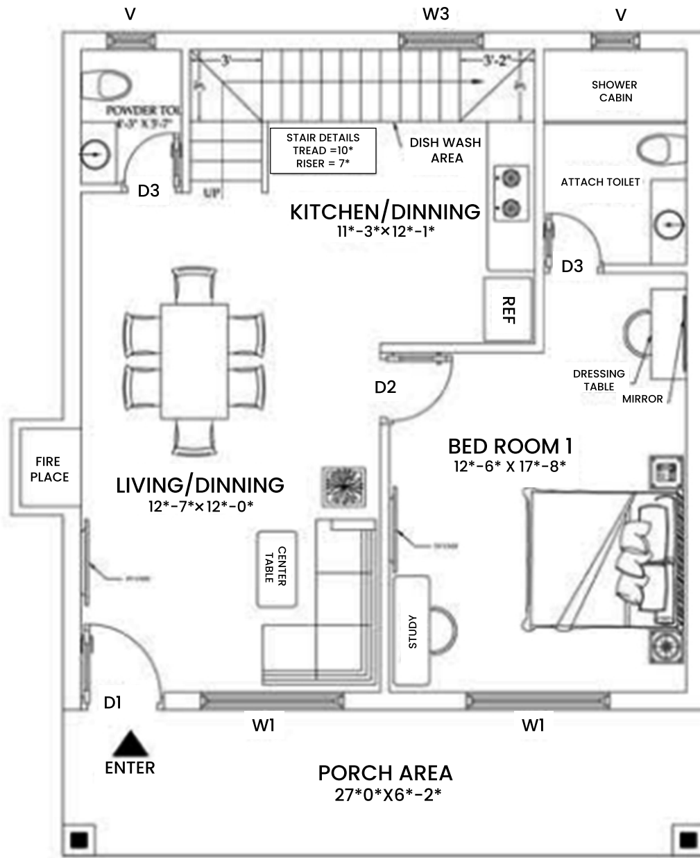
Ground Floor
