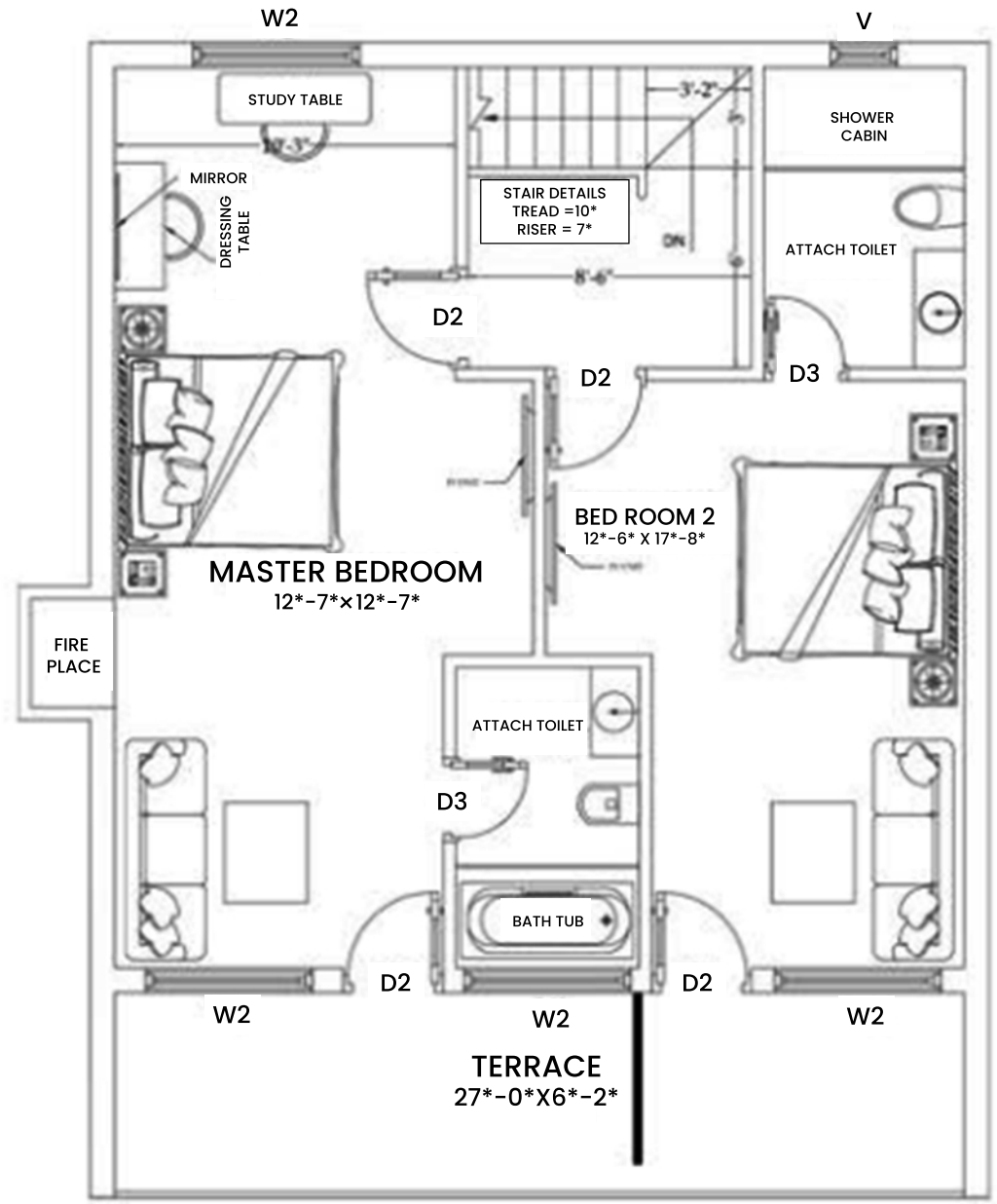
First Floor
